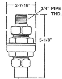
FIG. 5 VERTICAL STRAIGHT-THRU PATTERN (VST)
